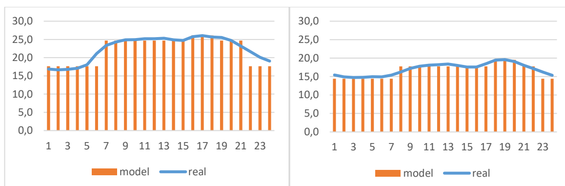
Figure 3. Real and model demand curve for winter - workdays (left) and weekends (right) in Poland [GW]
